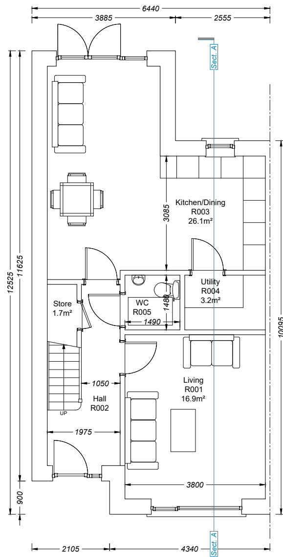
HOUSE TYPE: F FIRST FLOOR PLAN - 60.2M 2
