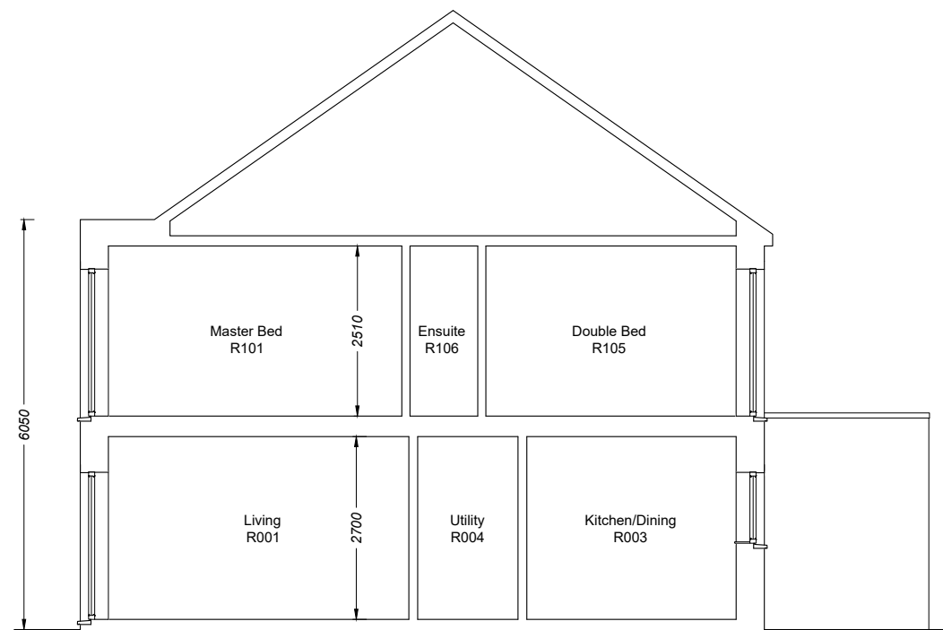
HOUSE TYPE: F SECTION AA
