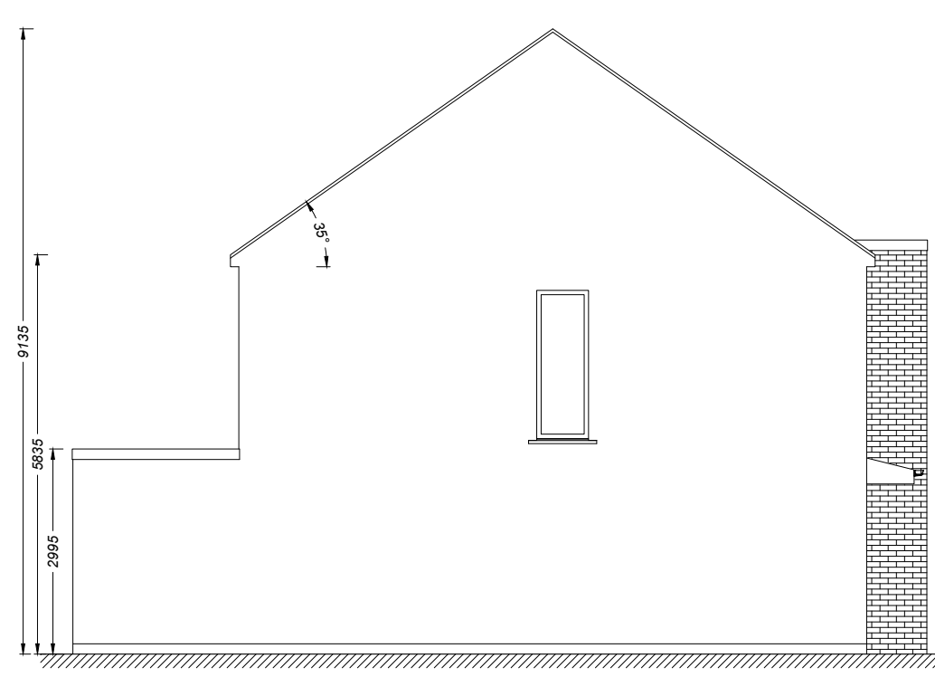
HOUSE TYPE: F SIDE ELEVATION
