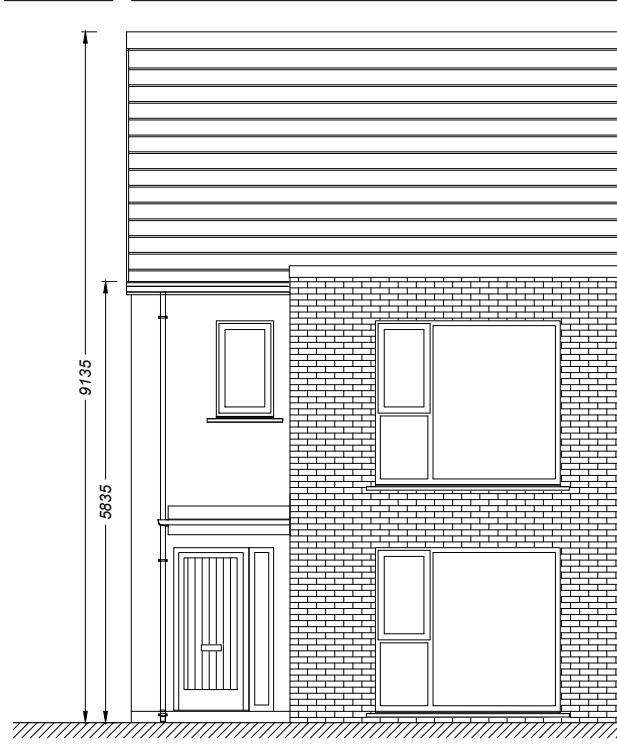
HOUSE TYPE: F FRONT ELEVATION
