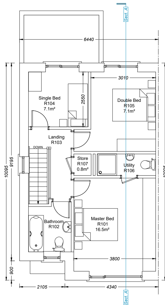
HOUSE TYPE: F FIRST FLOOR PLAN - 52.8M 2
